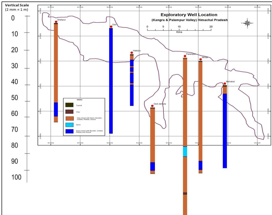
Fig.1.3 (b) The diagram showing disposition of aquifers
